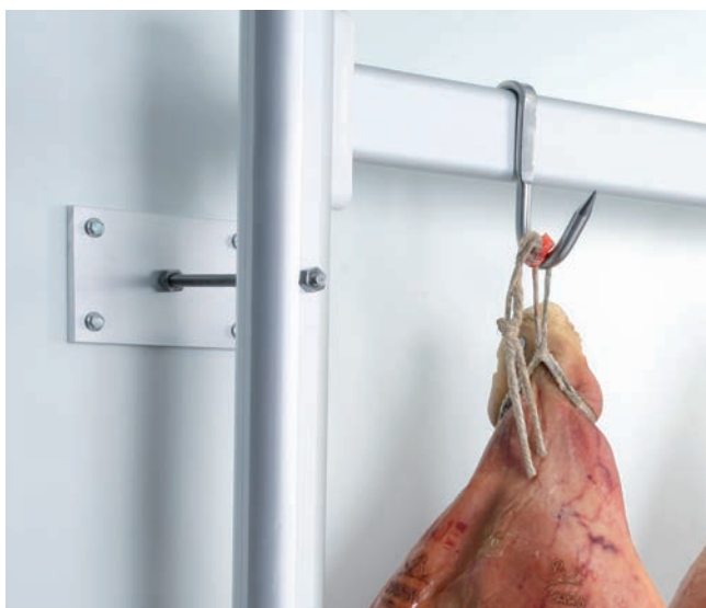
Gancera su piantane. Portata 50÷200 kg/m Hooked bar mounted on uprights. Load capacity 50÷200 kg/m
